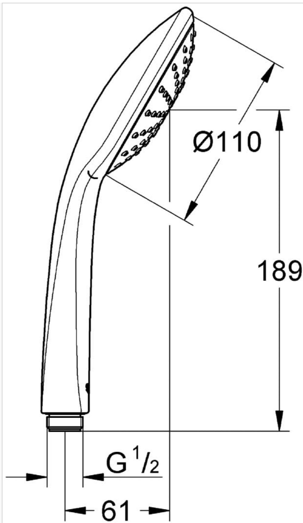
Image 4.1: Technical diagram illustrating the dimensions (in mm) and the standard G 1/2 inch connection thread for installation.
