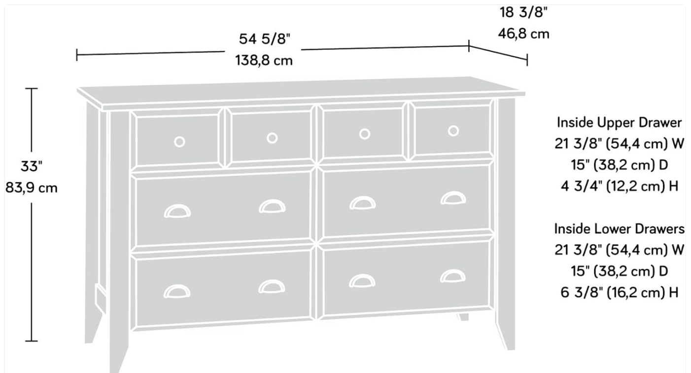
Figure 3.1: Dimensional diagram of the dresser, indicating overall dimensions and internal drawer measurements for both upper and lower drawers.
