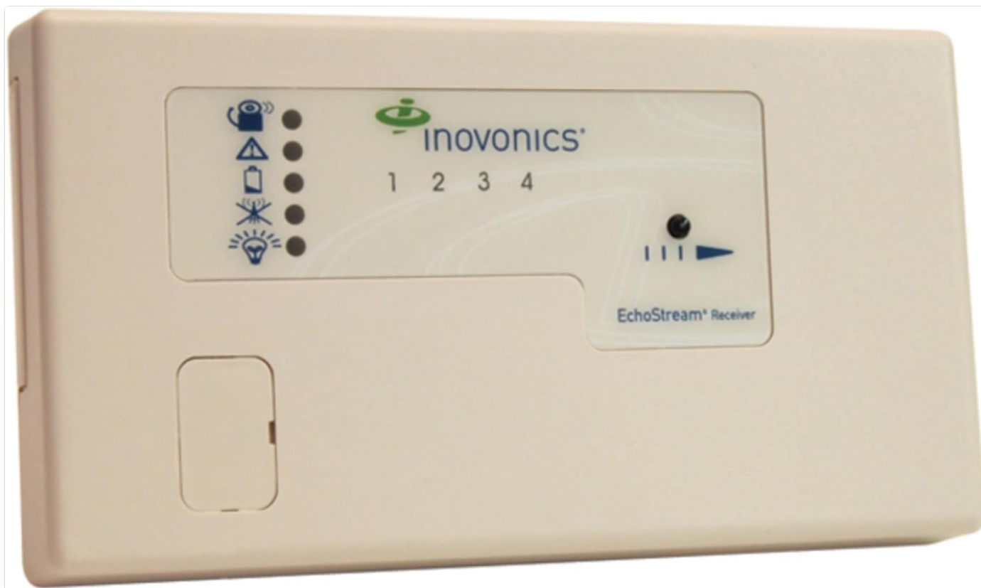
Figure 1: Front view of the Inovonics EN4204R 4-Point/5-Relay Output Receiver. The device features a light-colored casing with a clear panel displaying the Inovonics logo, four numbered indicators (1-4), and various status icons including signal strength, alert, and power indicators. A small, rectangular access panel is visible on the lower left.
