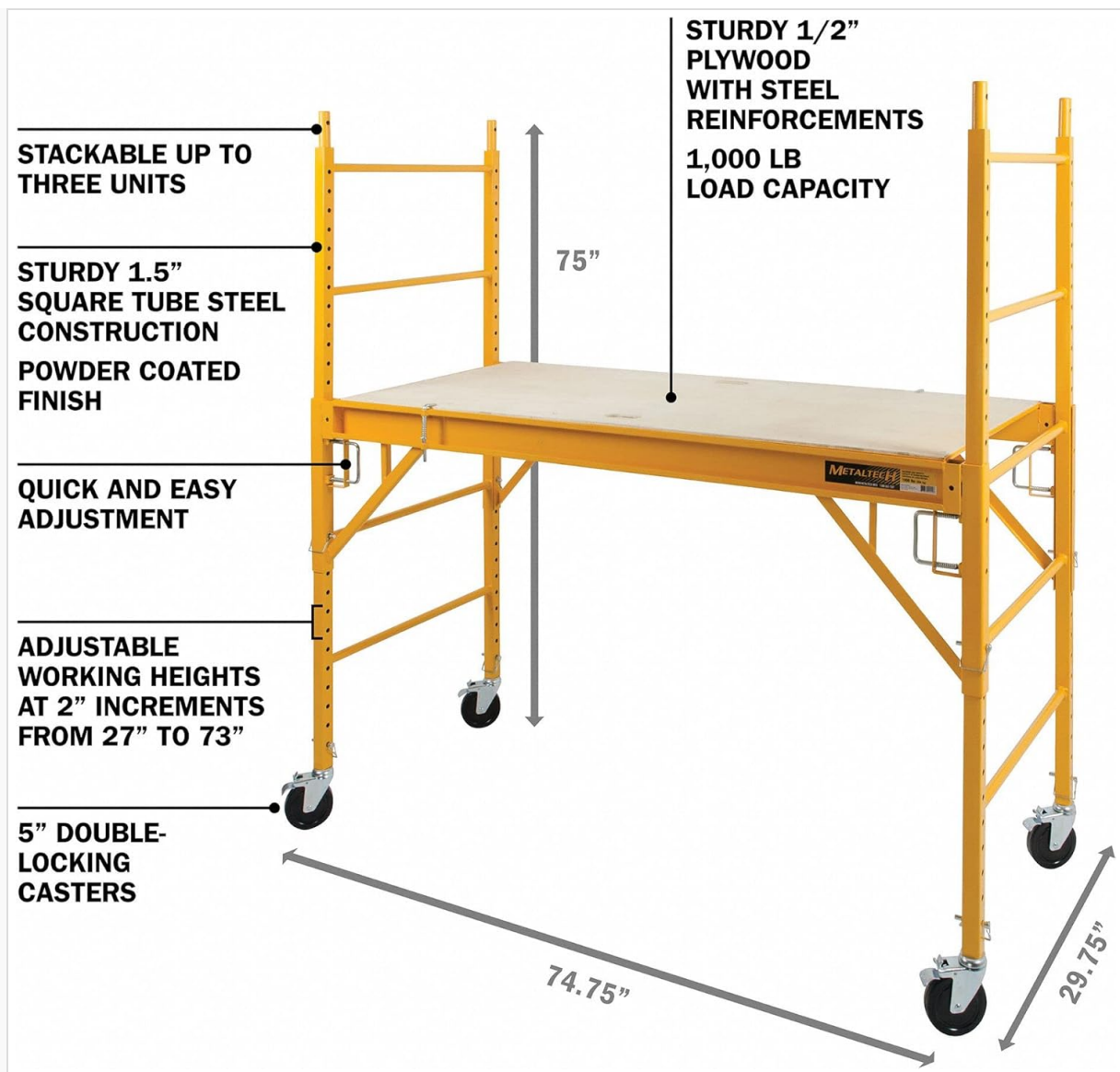
Figure 2.2: Detailed diagram illustrating the dimensions, load capacity, and adjustable features of the scaffolding platform.
