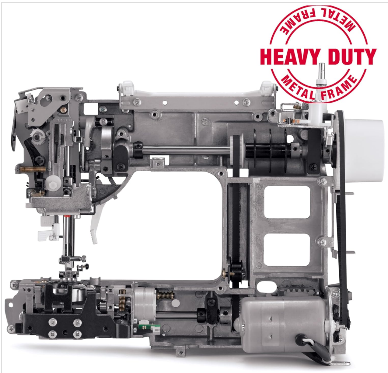
Figure 3.2: Heavy Duty Metal Frame. This image showcases the robust internal metal frame, emphasizing the machine's durability.
