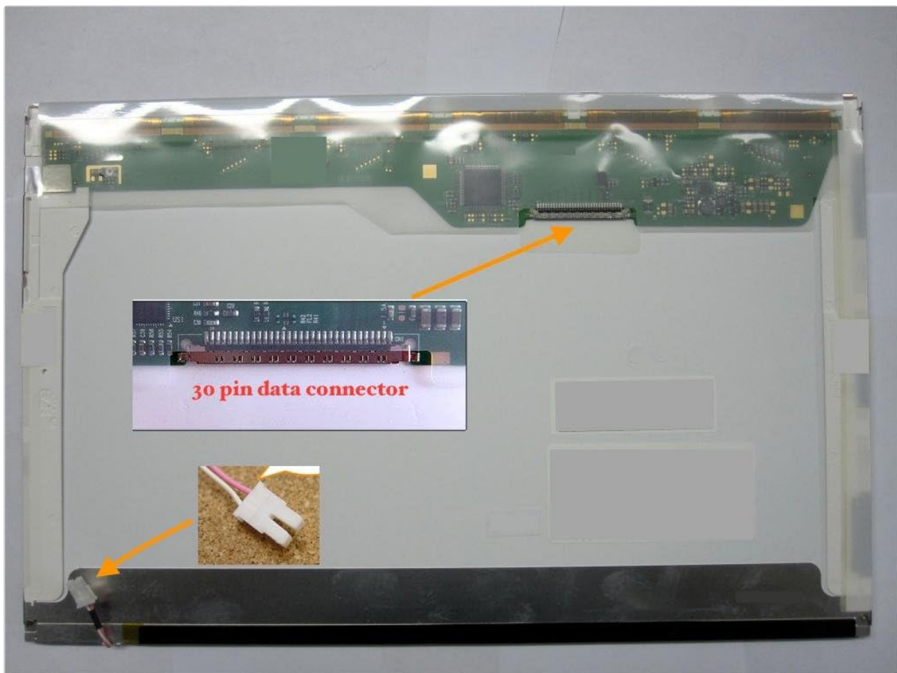
Figure 2.4: Detailed back view, indicating the location of the 30-pin data connector and the CCFL lamp connection.
