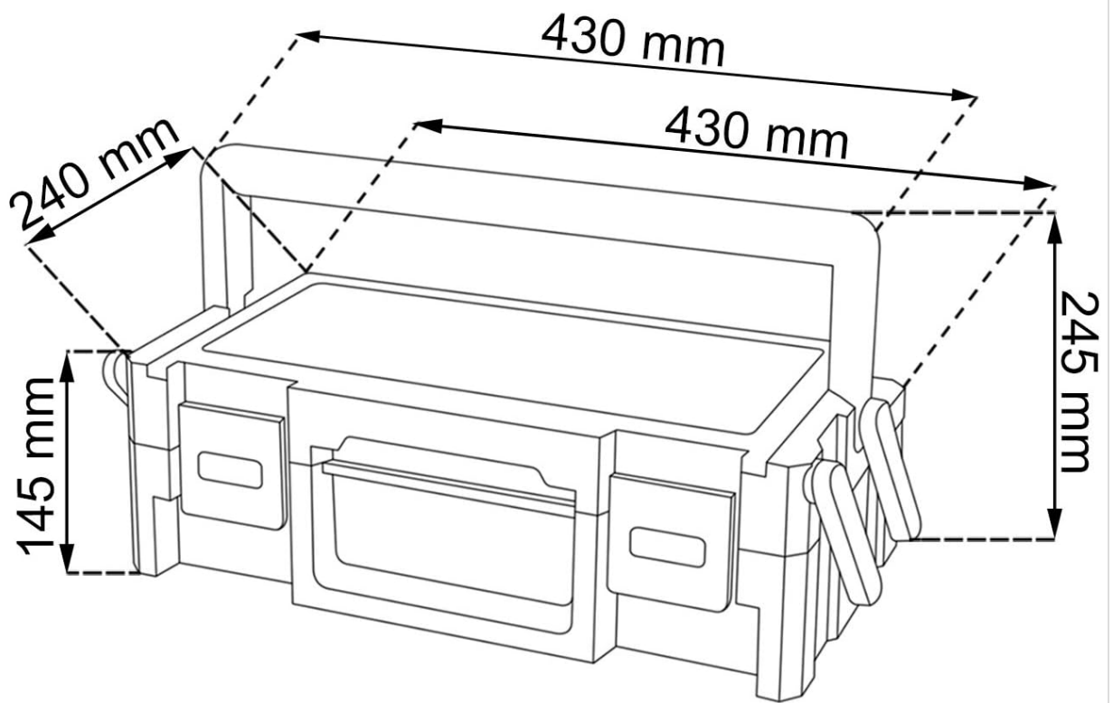
Figure 5: Overall dimensions of the Keter Master Pro Series Cantilever Assortment Box.
