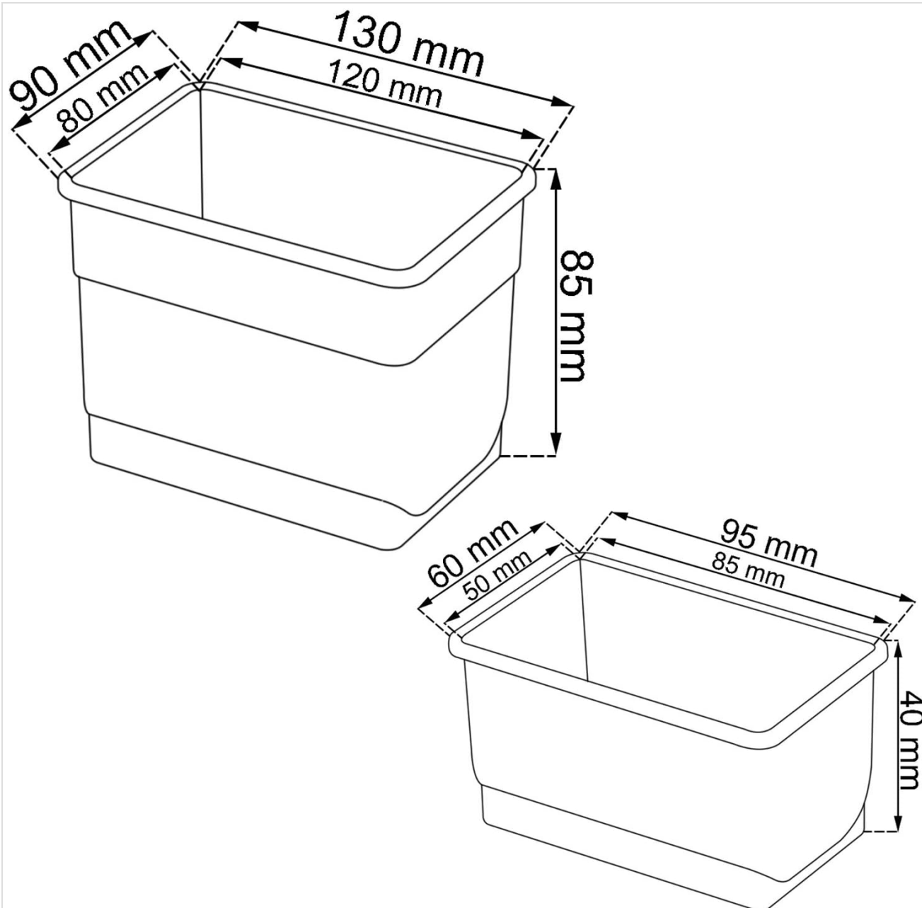
Figure 6: Dimensions of the two types of removable compartments.
