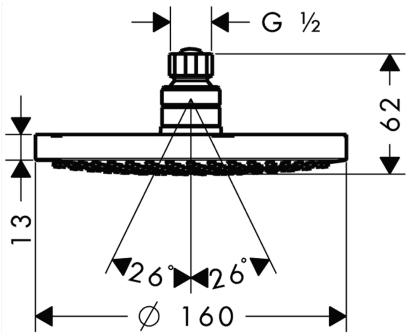
Figure 2: Technical drawing illustrating the dimensions of the Hansgrohe Croma 160 Overhead Shower. Key dimensions include a 160mm diameter, a total height of 62mm from the connection point to the bottom of the shower head, and a G 1/2 connection thread.
