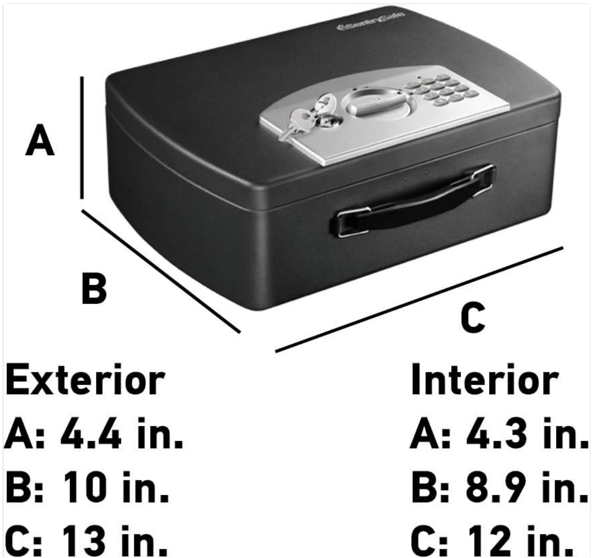
Image: Diagram illustrating the exterior and interior dimensions of the SentrySafe P021E Portable Safe Box.
