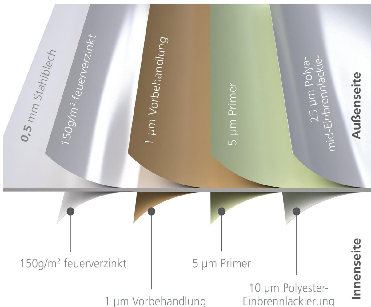
Image 3: Illustration of the multi-layer material construction for durability and weather resistance.
