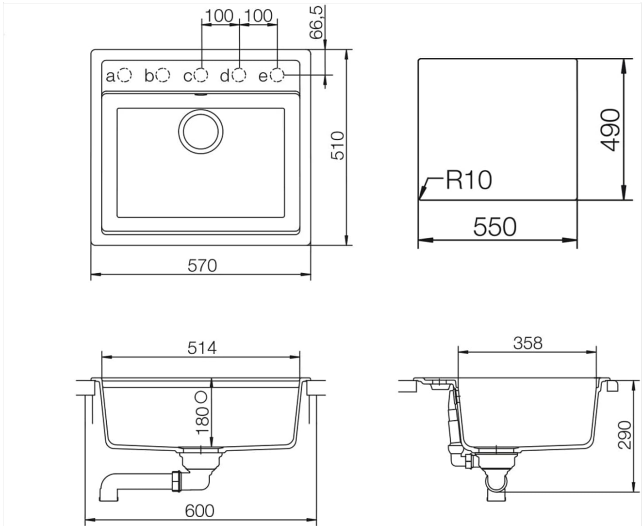
Image 2: Technical drawing showing precise dimensions and pre-drilled hole locations for installation.
