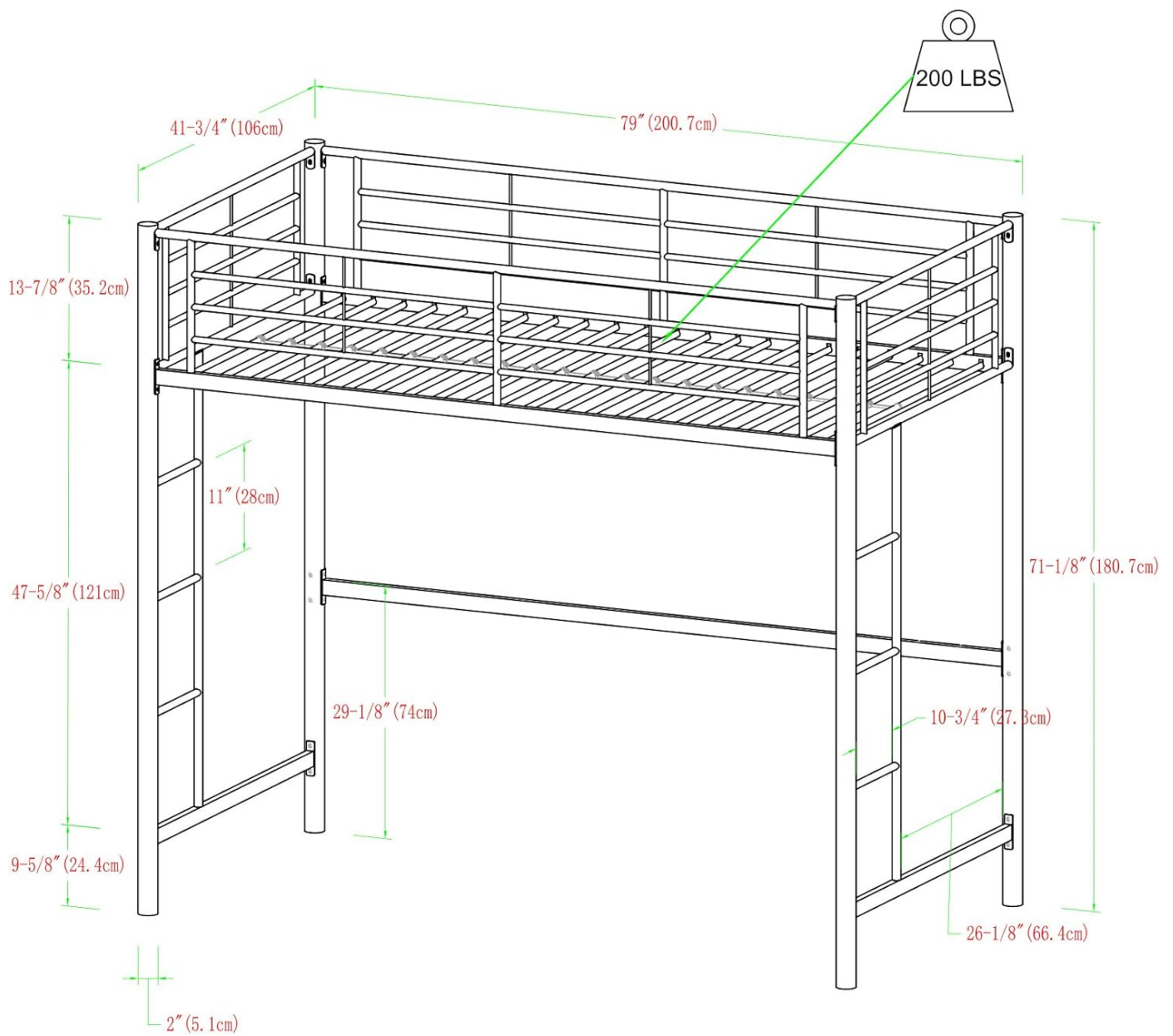
Image: Detailed diagram showing the dimensions of the Walker Edison Timothee Loft Bunk Bed.
