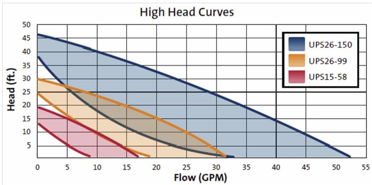
Figure 2: High Head Curves. This graph illustrates the performance characteristics of various Grundfos circulator pumps, including the UPS26-99, showing the relationship between flow rate (GPM) and head (feet).
