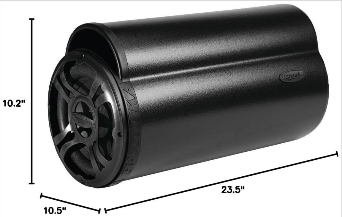
Image: Diagram showing the dimensions of the Bazooka BTA850FH subwoofer.
