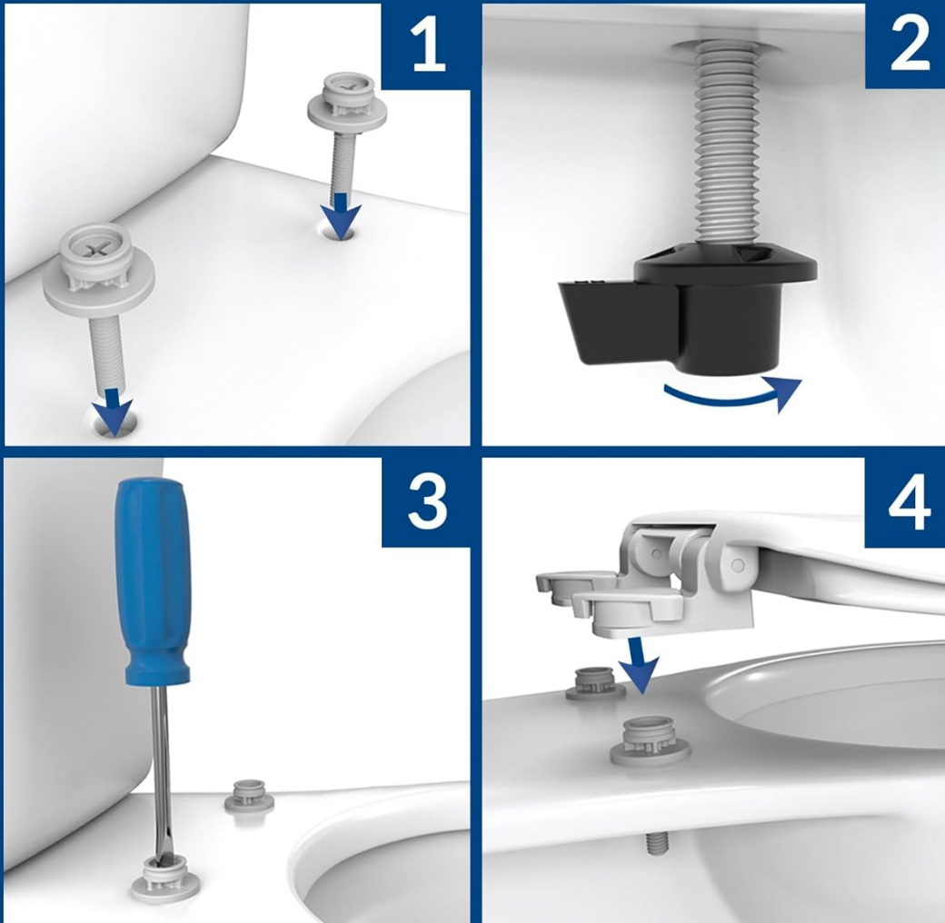
Image: A four-panel diagram illustrating the installation process: 1) inserting bolts, 2) securing nuts from below, 3) tightening with a screwdriver, and 4) attaching the seat to the secured bolts.
