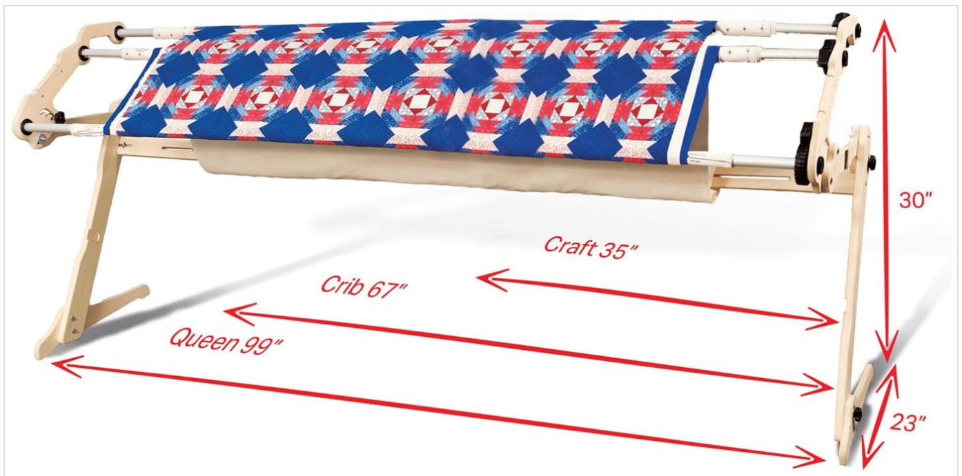
Image: The Grace EZ3 quilting frame displaying its adjustable lengths for Craft (35"), Crib (67"), and Queen (99") sized quilts, along with height (30") and depth (23") measurements.
