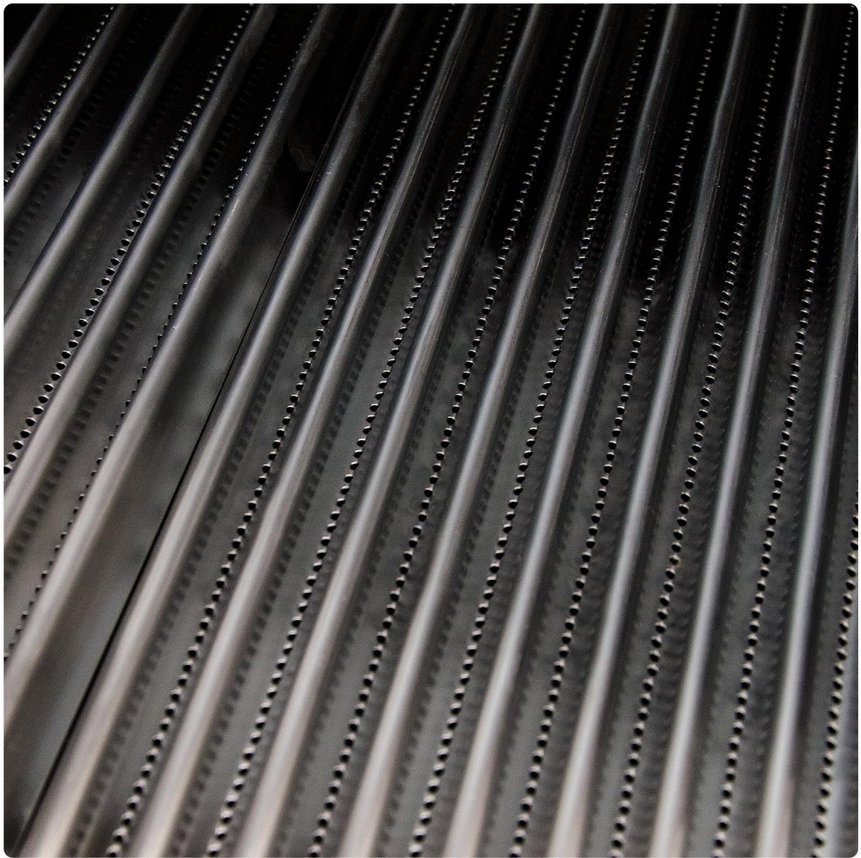
Figure 4: A detailed view of the unique corrugated stainless steel TRU-Infrared grates, designed for optimal heat distribution and cooking performance.
