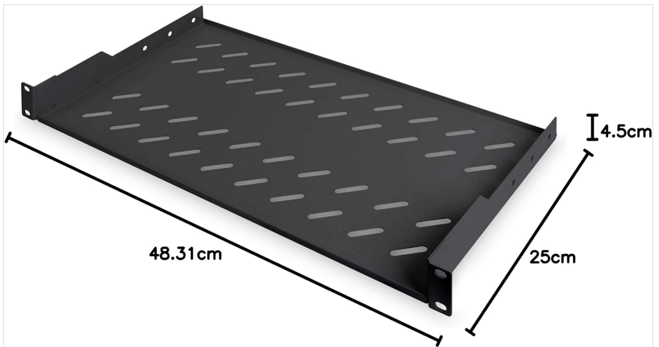
Figure 5: Detailed dimensions of the shelf: 48.31 cm width, 25 cm depth, 4.5 cm height.
