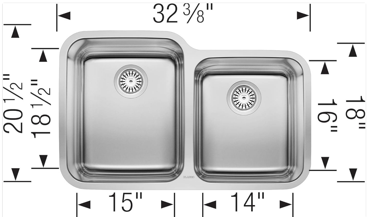
Image: Detailed dimensions of the BLANCO STELLAR 60/40 Double Bowl Undermount Kitchen Sink.
