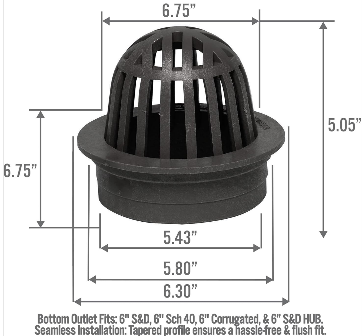
Figure 1: Dimensional view of the 6-inch atrium drain grate. This diagram illustrates the precise measurements for proper fitting into compatible drainage systems.
