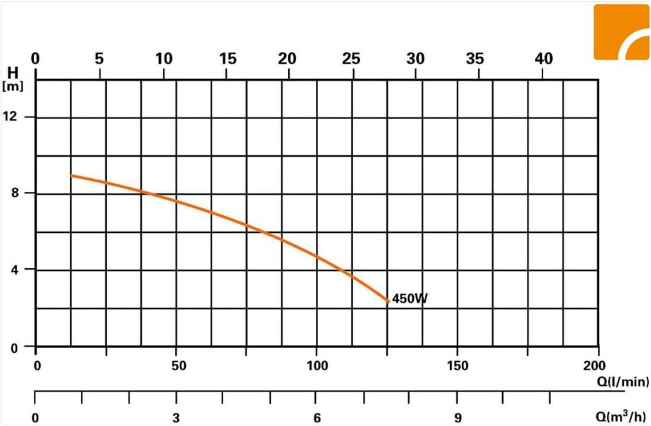
Figure 8.1: Pump Performance Curve.
