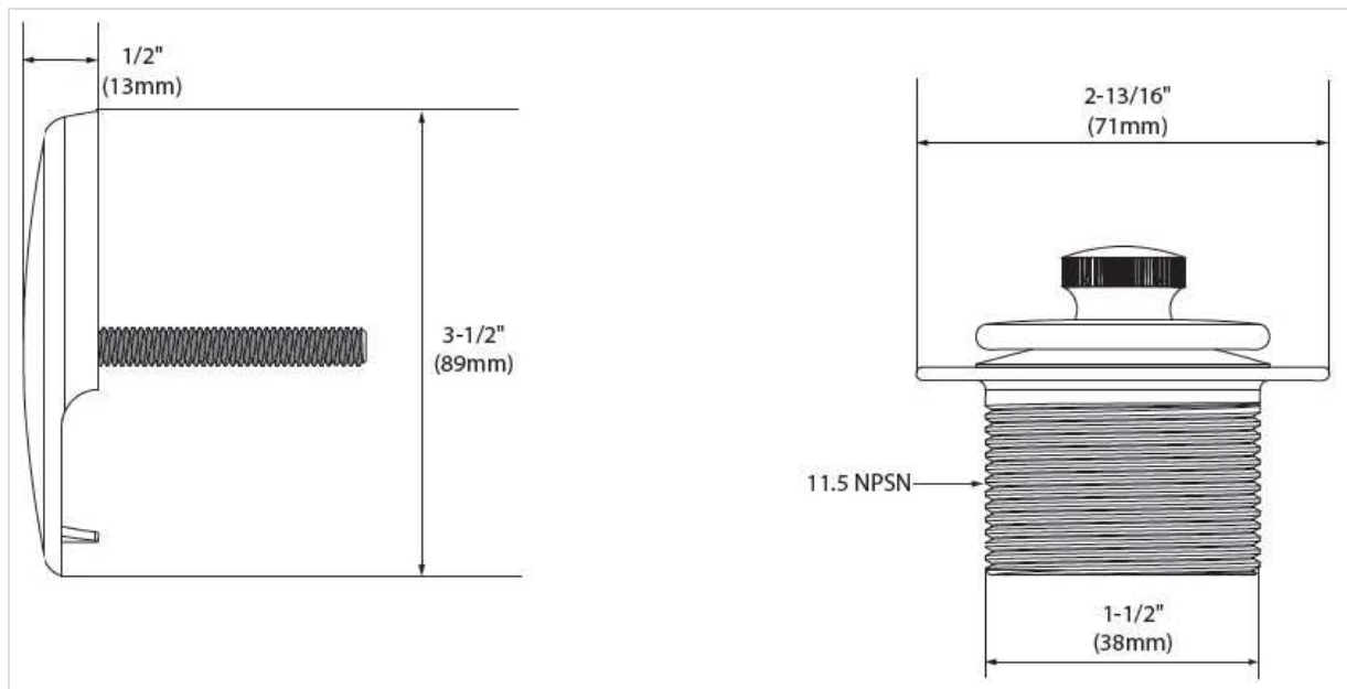
Image: Technical diagram illustrating the dimensions of the drain stopper (1-1/2 inch threads) and the overflow cover, providing critical measurements for installation.
