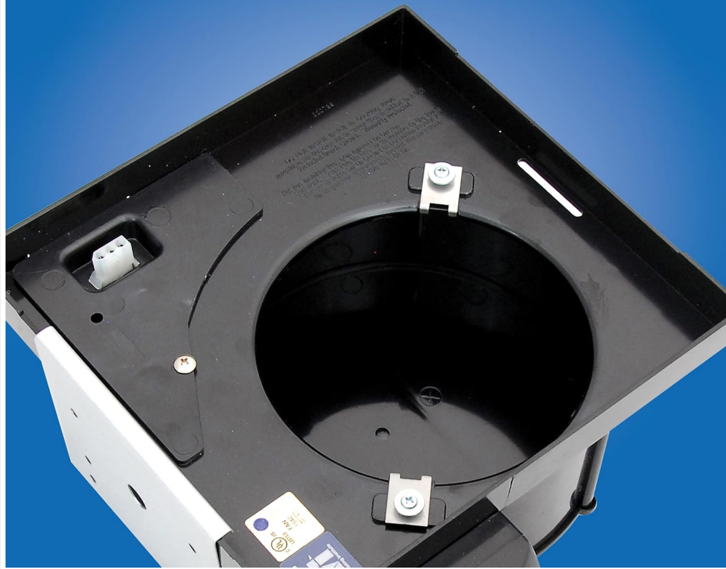
Figure 3.3: Standard 4" Round Duct Collar. This image highlights the 4-inch diameter of the fan's duct collar, indicating the required duct size for installation.
