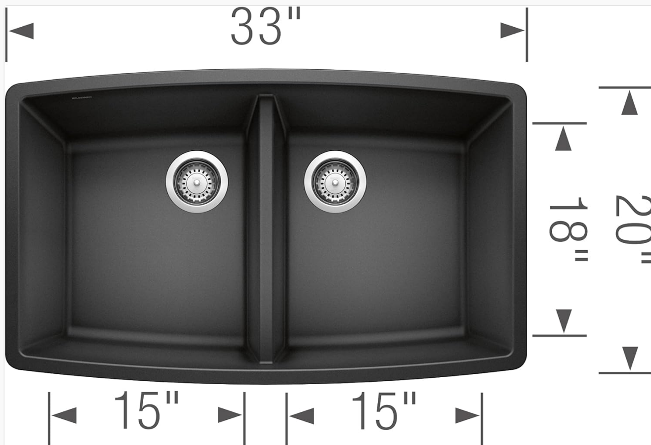
Figure 3: Detailed dimensions for the BLANCO PERFORMA 50/50 sink, including overall length (33"), width (20"), and individual bowl dimensions (15" x 18" x 10").
