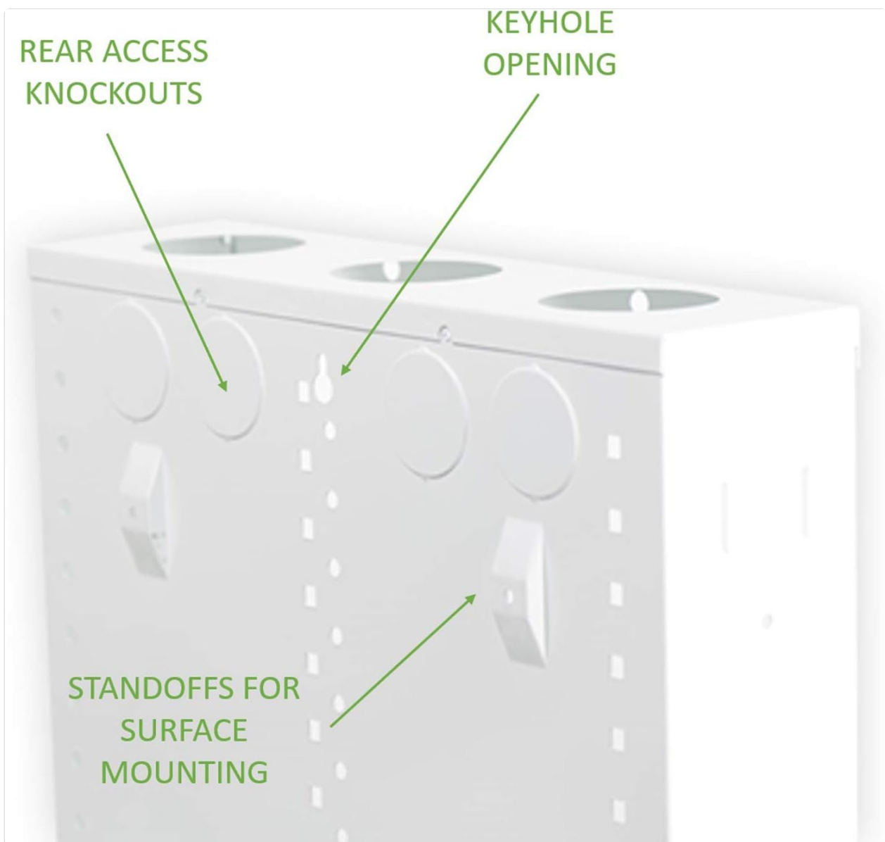
Figure 3.2: Details of the enclosure's rear access knockouts, keyhole opening for initial hanging, and standoffs for surface mounting.
