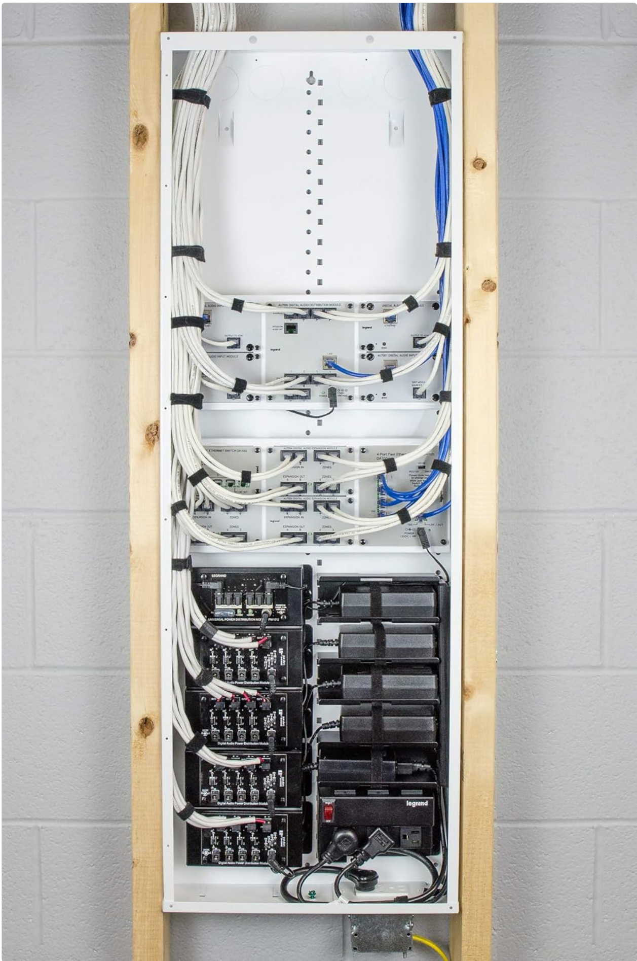
Figure 4.1: An example of a fully populated On-Q enclosure, demonstrating organized cabling and various installed modules for a structured wiring system.
