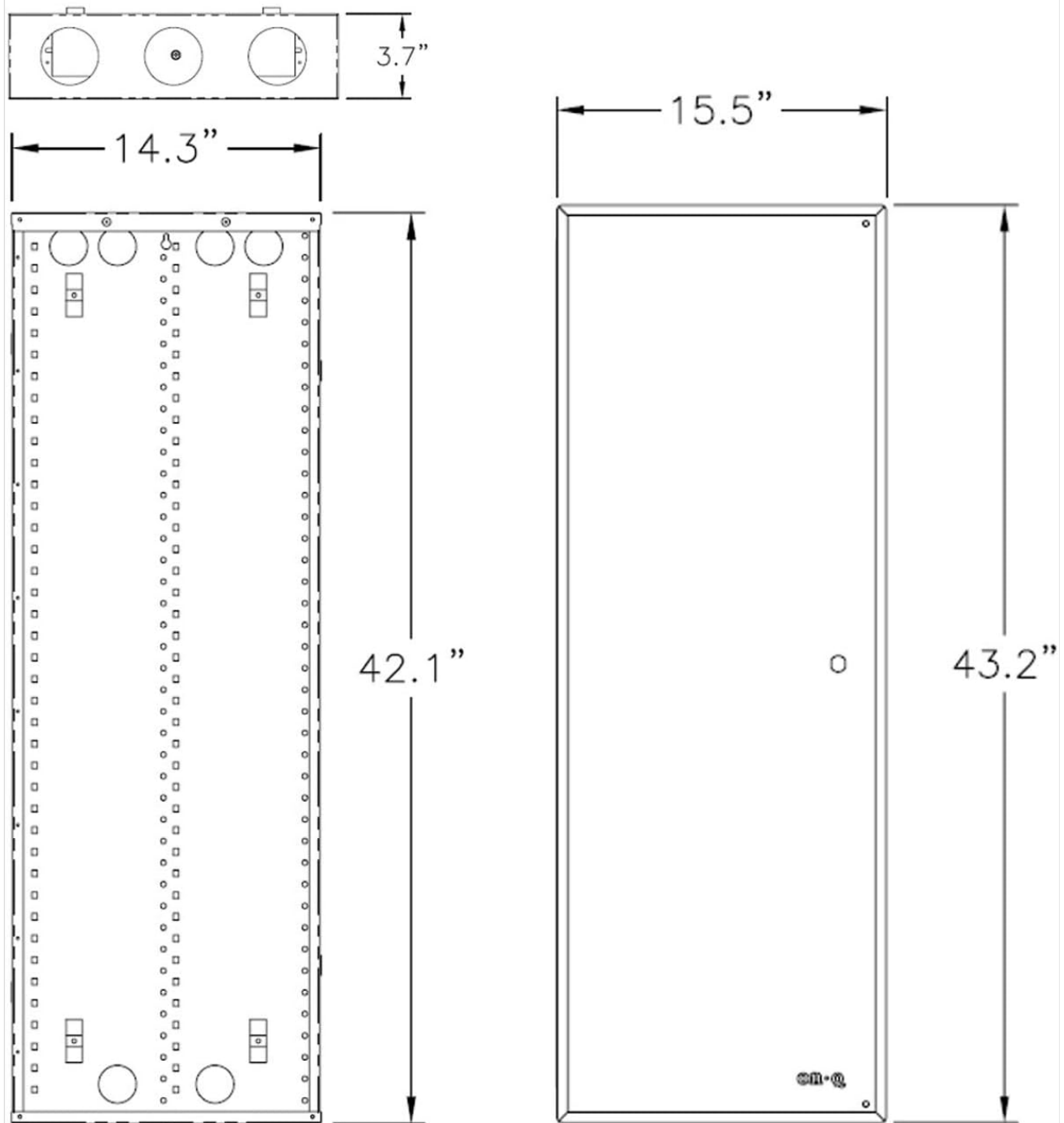
Figure 2.2: Detailed dimensions of the EN4250 enclosure, including depth, width, and height measurements for both the enclosure body and the hinged door.
