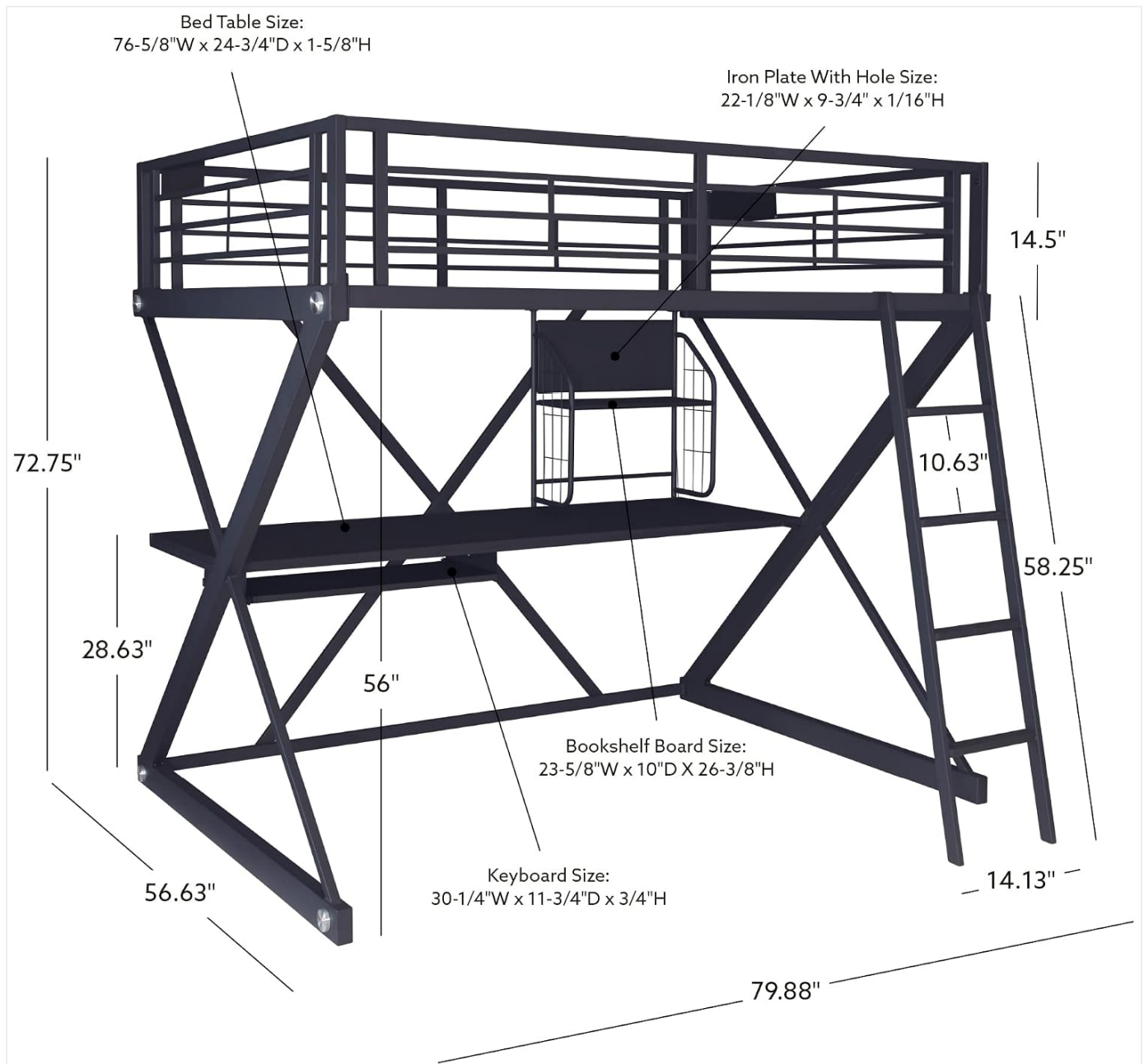
Image: A detailed diagram showing the dimensions of the Powell Z-Bedroom Loft Study Bunk Bed, including overall height, length, width, and specific measurements for the desk, keyboard tray, and bookshelf board.
