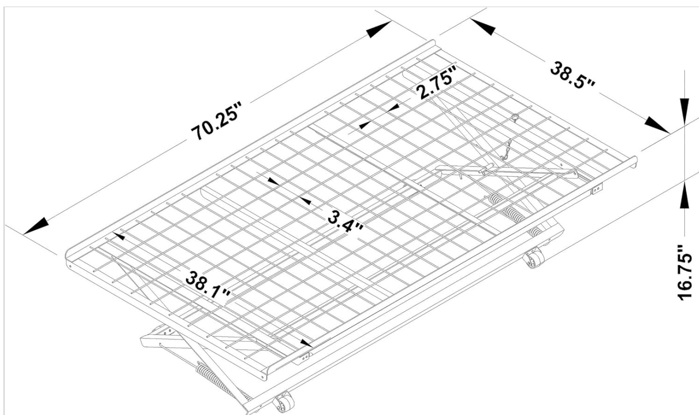
Figure 2: Detailed dimensions of the trundle, indicating a length of 70.25 inches, width of 38.5 inches, and a height of 16.75 inches when raised. The collapsed height is approximately 6 inches. These measurements are crucial for ensuring compatibility with existing bed frames and mattresses.
