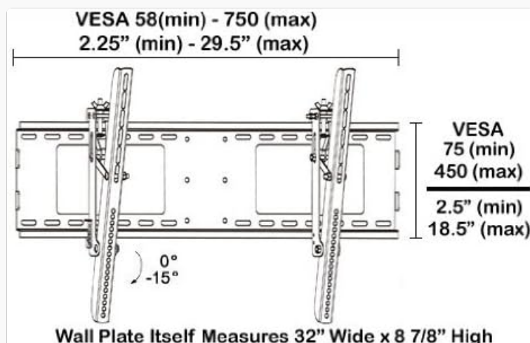
Image 2: Diagram illustrating the Brateck WALLM14-1704 wall mount's dimensions, including VESA ranges (horizontal 58-750mm, vertical 75-450mm) and the 0° to -15° tilt capability. The wall plate dimensions are also shown.
