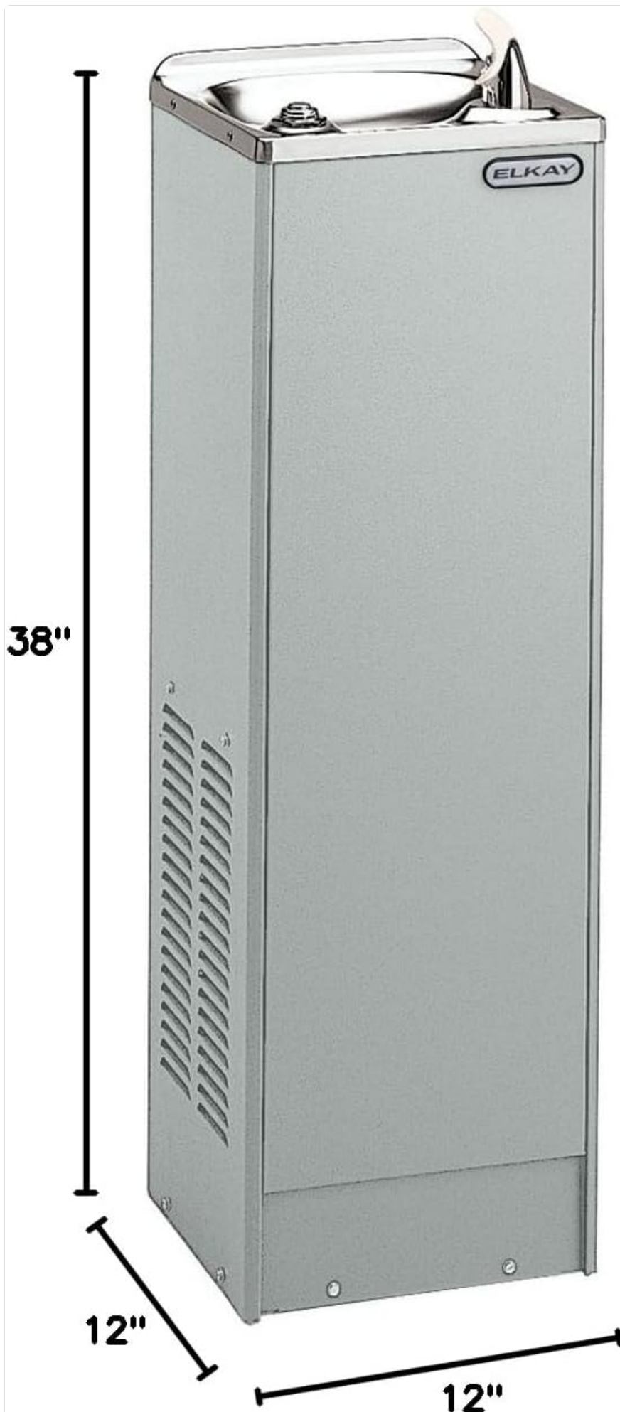
Figure 2: Dimensions of the Elkay FD7003L1Z Space-ette Cooler.
