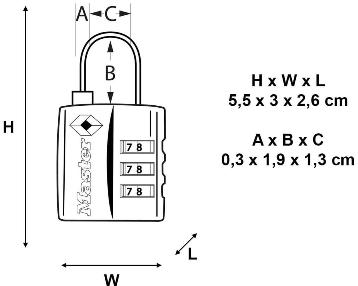
Image: Technical diagram illustrating the height (H), width (W), length (L) of the lock body, and the shackle dimensions (A, B, C) with corresponding measurements.
