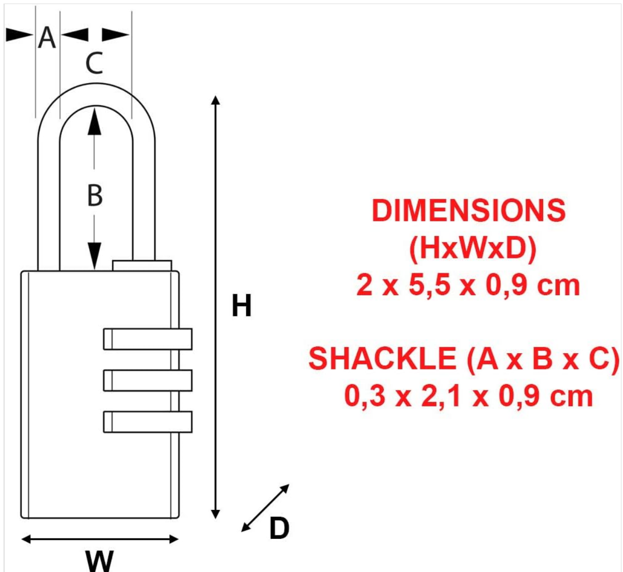
Figure 4: Dimensional diagram of the padlock.
