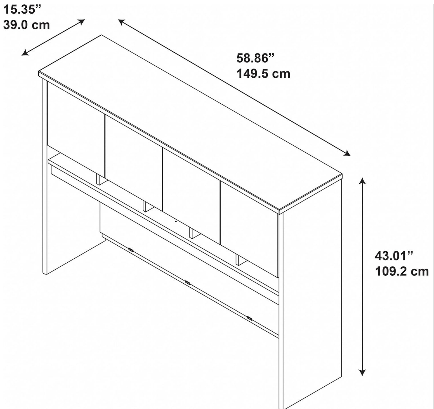
Image 3.1: Dimensional diagram of the 60W Hutch, showing height, width, and depth measurements for planning and assembly.
