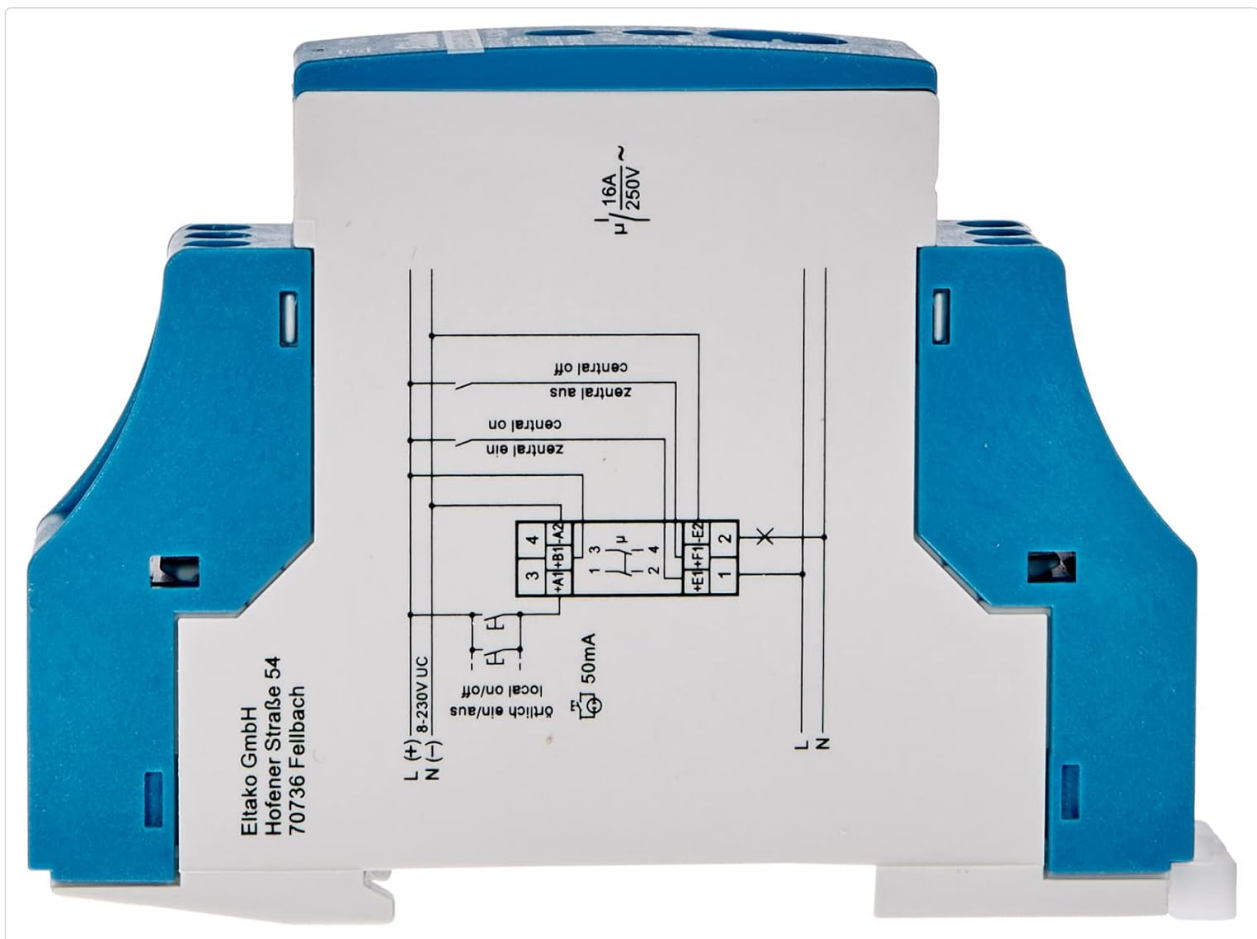
Image 1: Wiring diagram for the Eltako ES12Z-200 impulse relay. This diagram illustrates the connections for the main power supply (L, N), local control input, centralized control inputs (central on, central off), and the output contacts (1, 2). It also shows the internal circuitry for the control voltage and the 16A/250V output rating.
