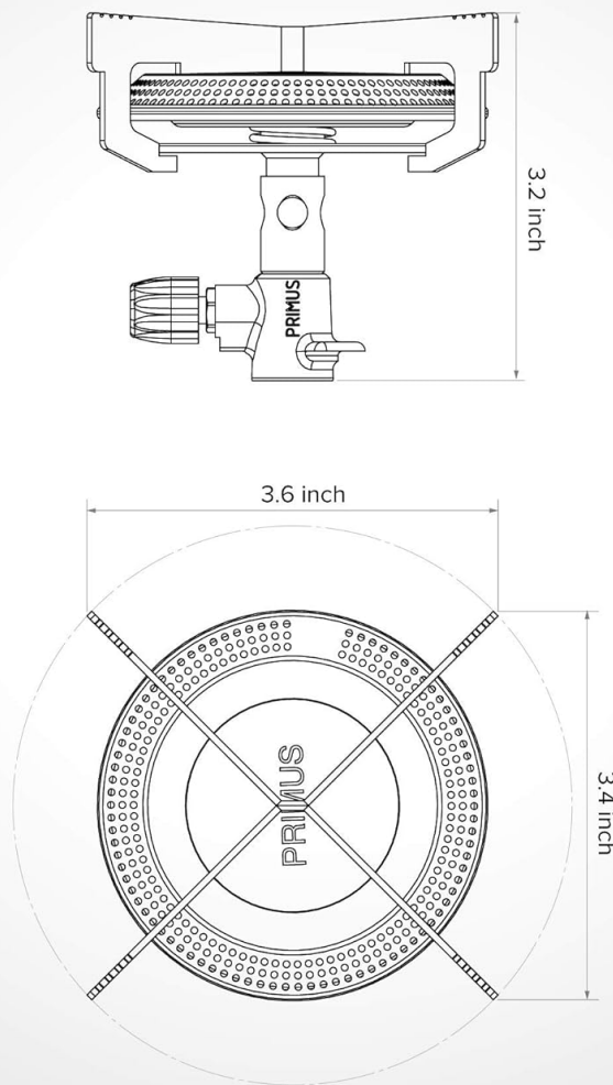
Image 5: Detailed dimensions of the Primus Classic Trail Stove.
