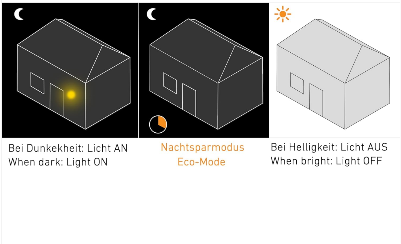
Figure 5.1: Illustration of the NightMatic 3000's automatic lighting functionality. It depicts light turning on when dark, an eco-mode period, and light turning off when bright.
