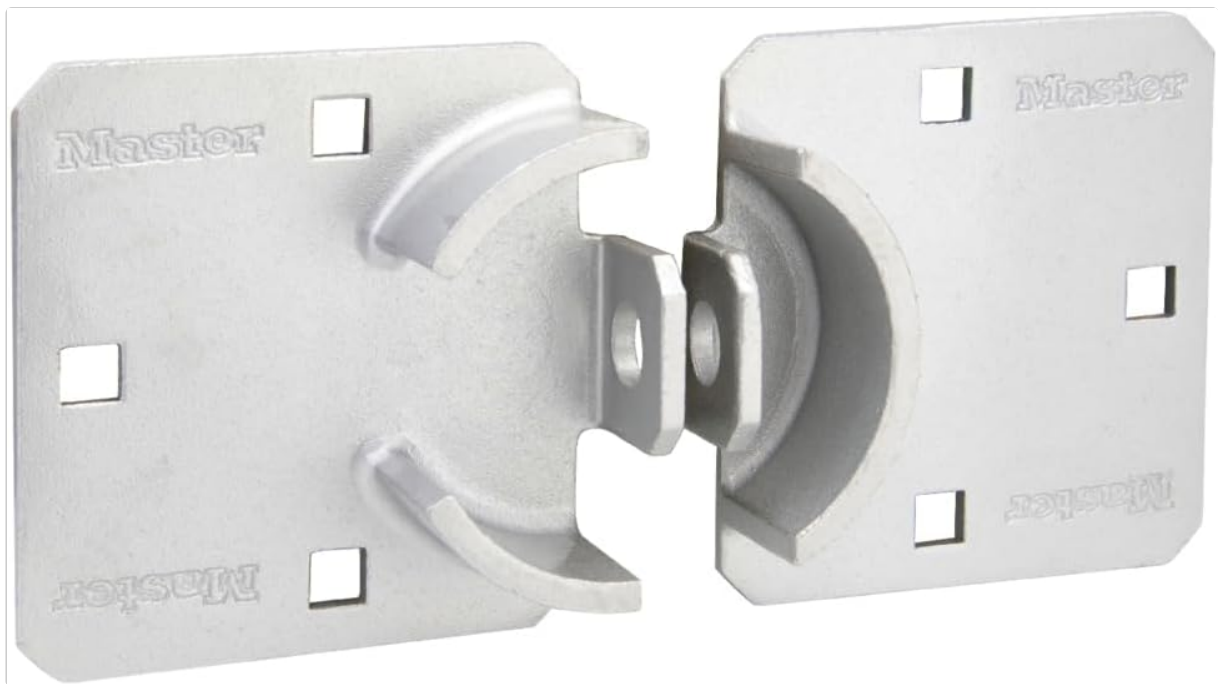
Image 2.1: Front view of the Master Lock Model 770 Hidden Shackle Hasp. This image displays the two main components of the hasp, designed to interlock and enclose a padlock shackle for enhanced security.
