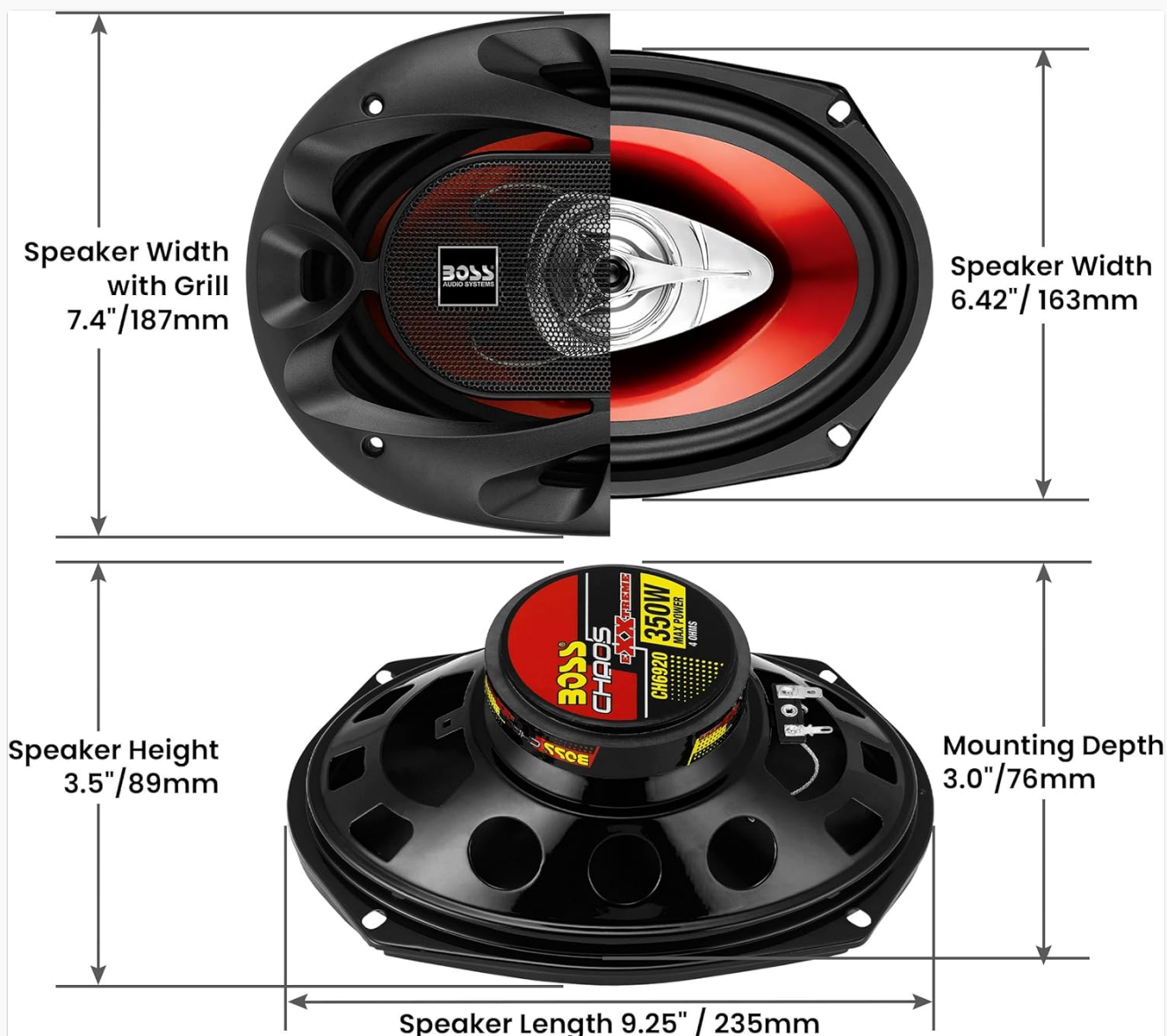
Figure 4.1: BOSS Audio Systems CH6930 Speaker Dimensions.
