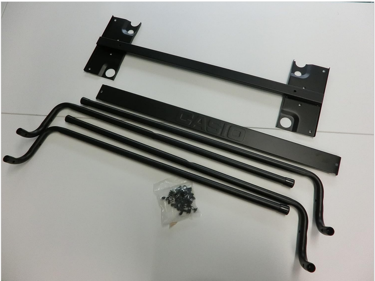
Image: All components of the CASIO CS-4B stand laid out, including the top support frame, legs, and connecting hardware.
