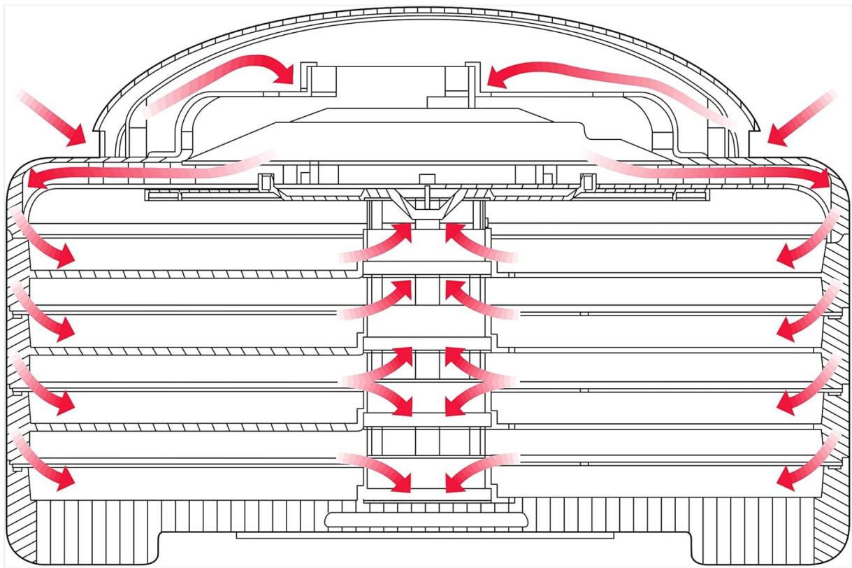
A diagram illustrating the Converga-Flow air circulation system within the Nesco dehydrator. Red arrows show how heated air is distributed evenly across all trays, ensuring consistent drying.
