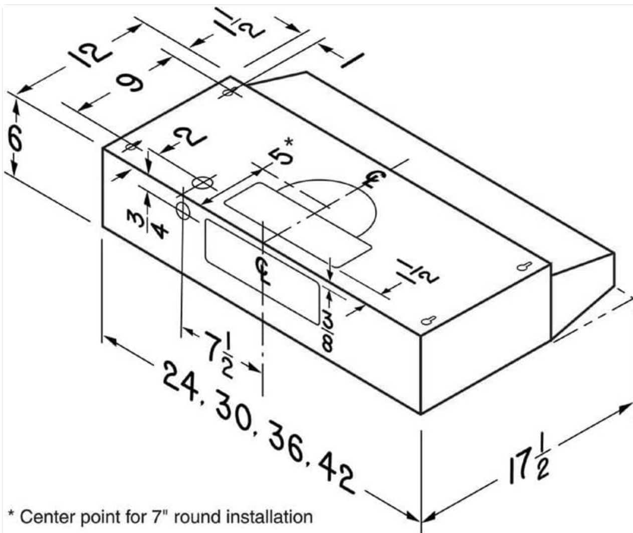
Figure 3: Dimensional drawing of the range hood, indicating width, depth, and height for various models.
