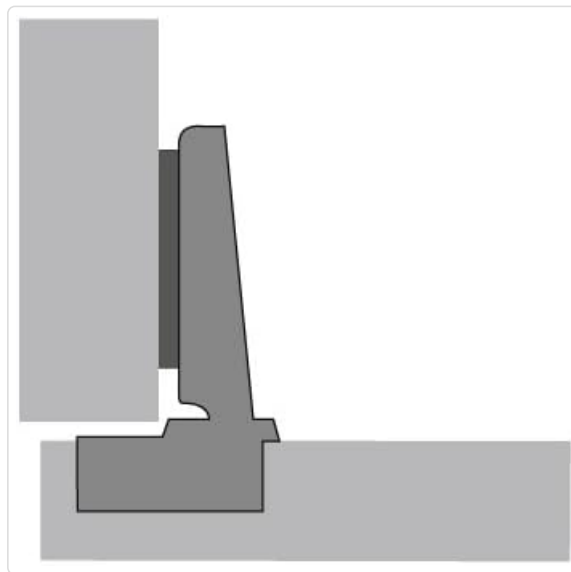
Image: Diagram illustrating the 52mm / 2.05 inch spacing for mounting plate screws, relevant for screw-on applications.
