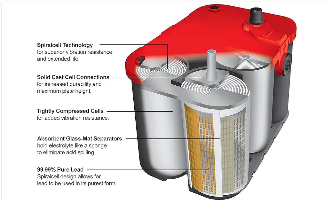
Image 6.1: OPTIMA RedTop Battery in a typical usage environment.
