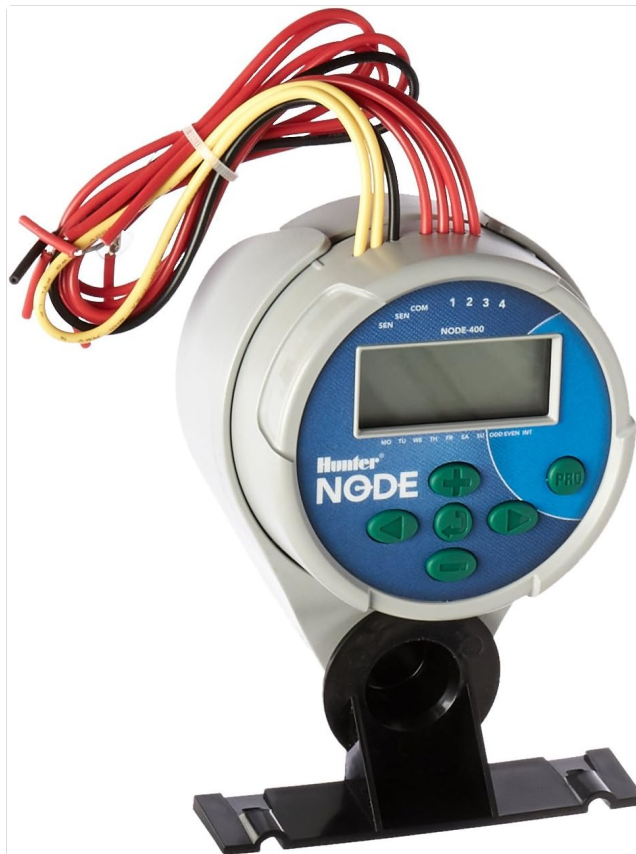
Image: Hunter Node400 controller shown with an optional mounting bracket, illustrating how the unit can be secured within a valve box for stable installation.
