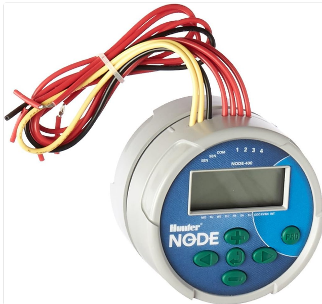
Image: Front view of the Hunter Node400 controller, displaying the LCD screen, control buttons, and the colored wiring harness for connecting to irrigation stations.
