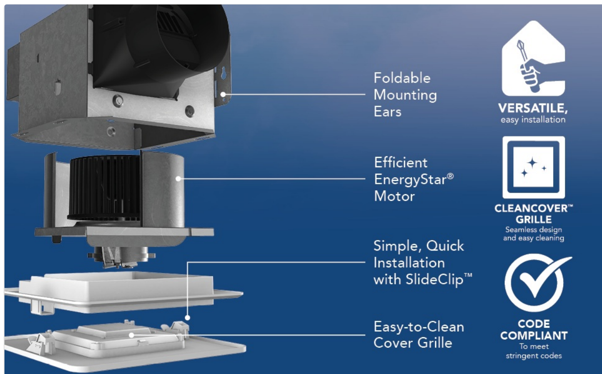
Figure 3: Exploded view highlighting internal components and mounting features.
