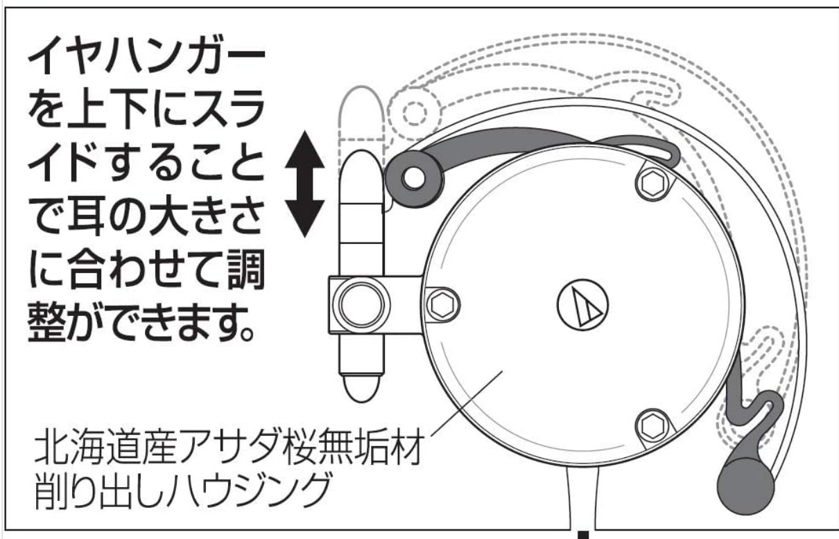
Figure 2: Diagram showing the adjustable slide-fit mechanism and rubber support for the ear hangers, allowing for a customized fit.
