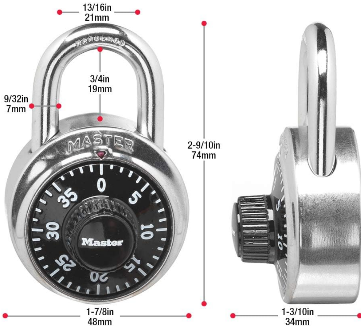
Image: Detailed dimensional drawing of the Master Lock 1500T, showing key measurements of the lock body and shackle.
