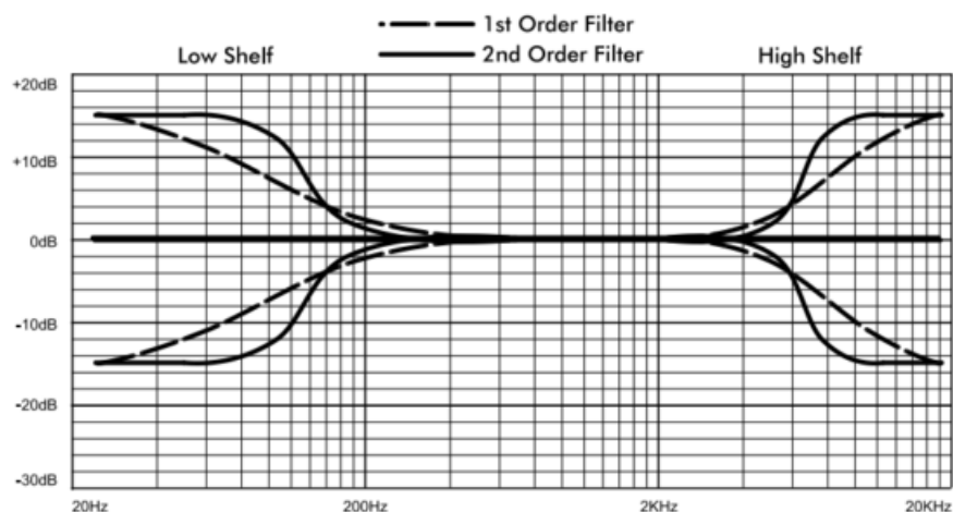
4.8SP and 3.6SP Shelving Filters
