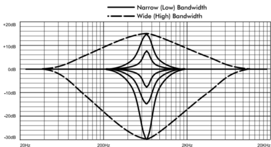
4.8SP and 3.6SP Parametric Filters
