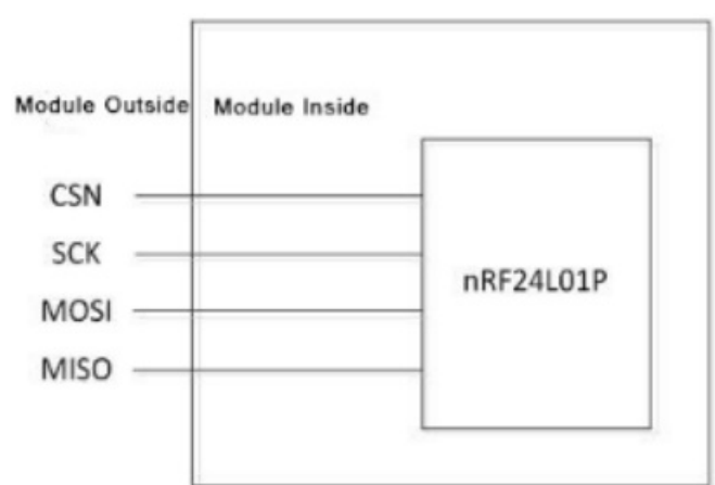
Picture 5-4 SPI Local Connection Diagram
