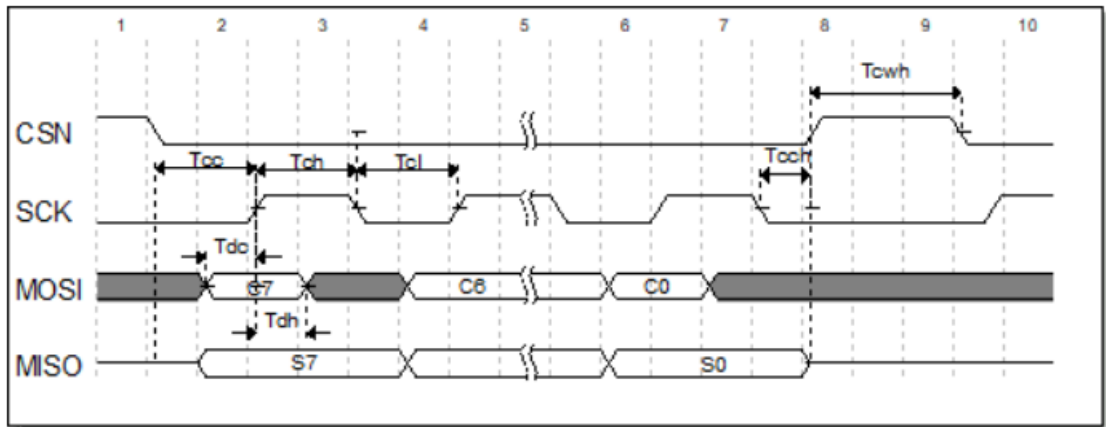
Picture 5-7 SPI Sequence Diagram of Parameters
