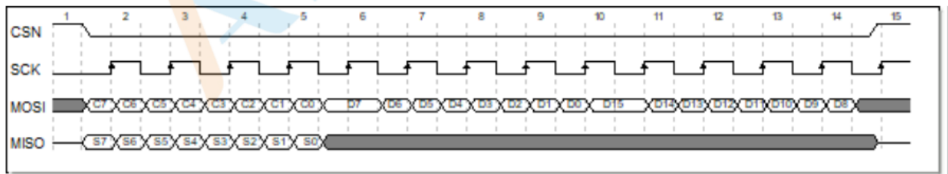
Picture 5-6 Sequence Diagram of SPI Write Operation
