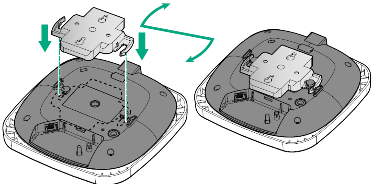
Figure 11 Bracket Installation
