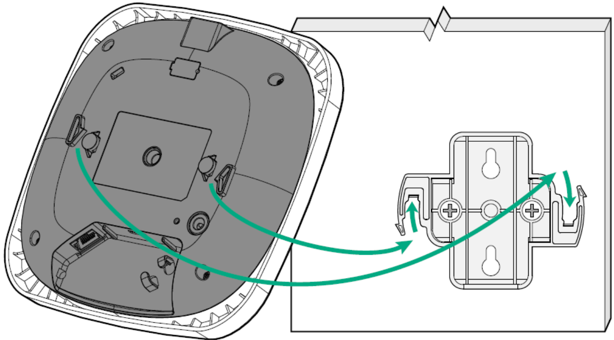
Figure 10 Attaching the AP to the Mount Bracket
