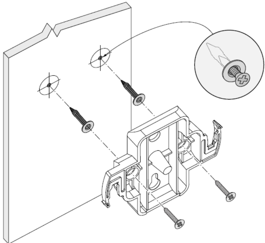
Figure 9 Attaching the Mount Bracket to a Solid Surface
