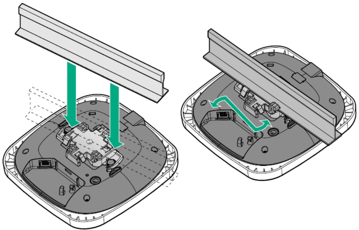
Figure 7 Mounting the AP to a 9/16" Ceiling Rail
