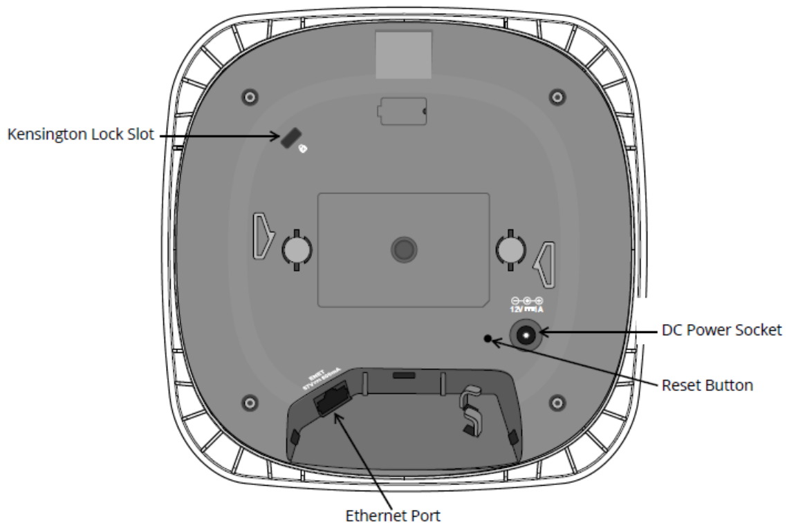
Figure 2 Back Panel
