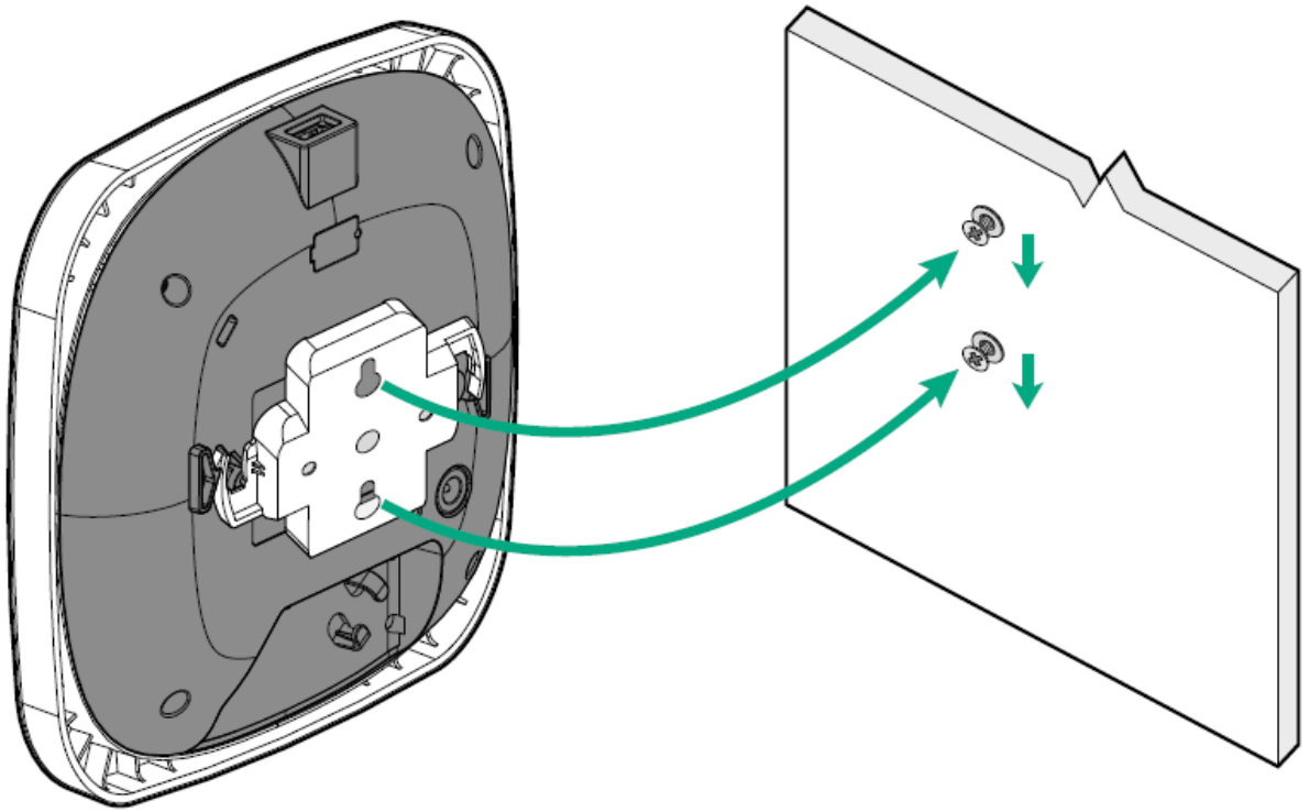
Figure 12 AP-Bracket Wall Installation
