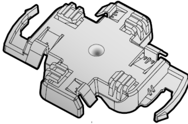
Figure 4 Ceiling Mount Bracket
