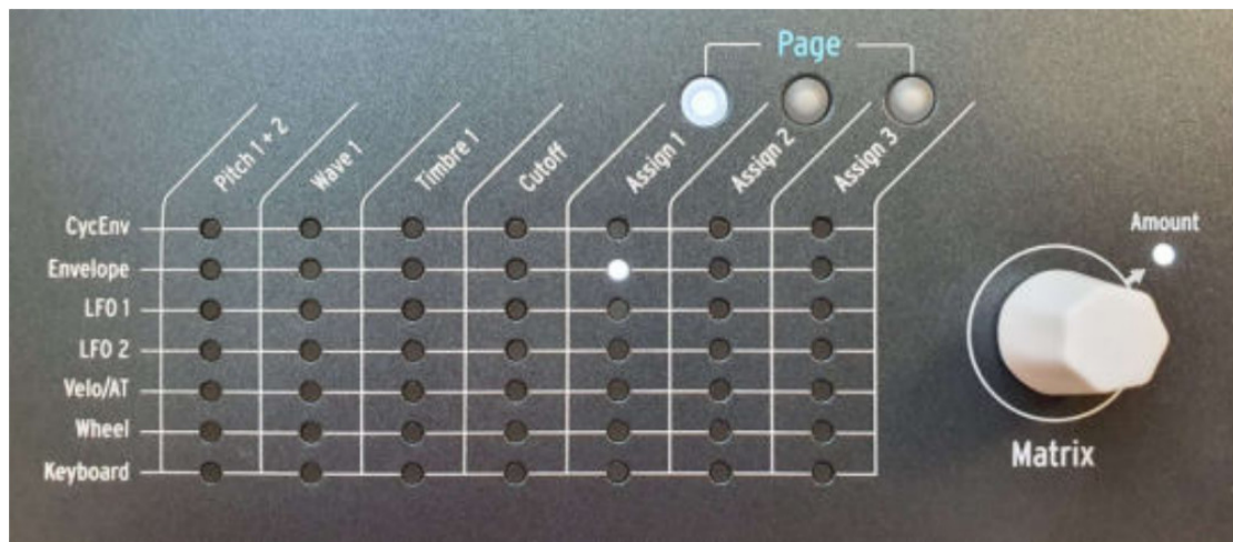
The Modulation Matrix
